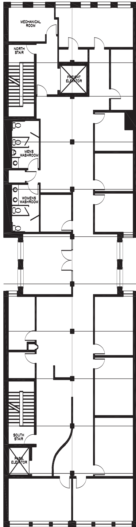
730 WEST RANDOLPH STREET SIXTH FLOOR PLAN
